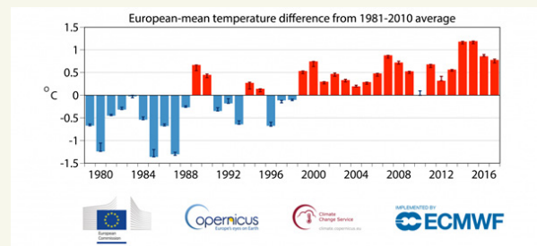
Fig. 4: Evolution of the mean air temperature in Europe (Source: https://climate.copernicus.eu/climate-2017-european-temperature ).
