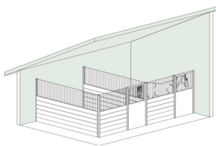
Innenbox 14.6%
