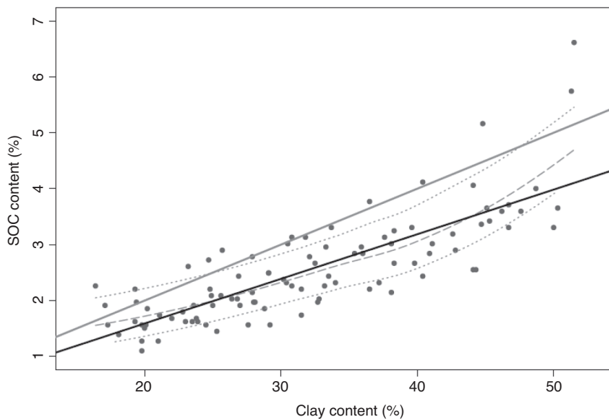
FIGURE 1 Linear model and ‘lowess’ nonparametric local regressions between soil organic carbon (SOC) and clay content; black solid line: linear regression line; light grey dashed line: lowess smooth curve (polynomial degree 2); light grey dotted lines: 95% confidence interval; grey solid line: 1:10 SOC:clay ratio; the parameters of the regression equations are given in Table 3.
