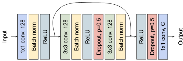
Fig. 3. Label refinement CNN architecture.
