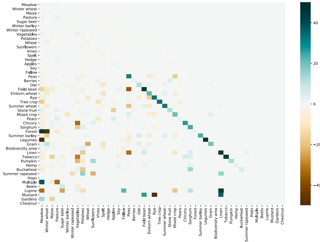
Fig. 7. Benefit of ms-convSTAR: Difference between normalized confusion matrices. Averaged over 5 cross-validation folds. Green denotes margins in favour of ms-convSTAR (higher correctness on the diagonal, respectively lower confusion off the diagonal), brown denotes margins in favour of the baseline counterpart (convSTAR). (For interpretation of the references to colour in this figure legend, the reader is referred to the web version of this article.)
