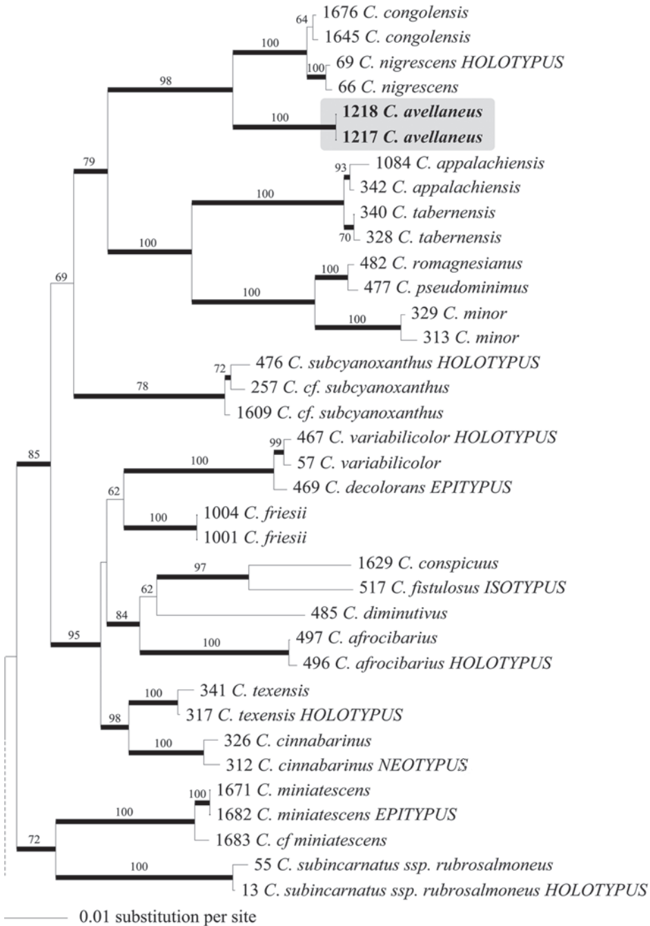
Fig. 1. Part of the most likely tree ( -\ln = 23582.653 ) inferred by phylogenetic analyses of the 4 locus-96 taxa alignment. Branches in bold received significant bootstrap values ( \geq 70\% ), which are reported along branches. Extractions 1217 and 1218 were obtained from different fruiting bodies, but generated identical sequences.
