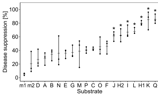
Figure 2. Disease suppression against P. ultimum of compost applications. Disease suppression was defined as the relative shoot weight of Pythium -inoculated compared with -uninoculated plants and calculated for each of the compost substrates and the control matrix in two batches. Control (m1 and m2) and compost treatments (A–Q) were ordered by their mean % disease suppression, and compost H was tested in both batches (H1 and H2) to assess the interbatch variability. Dashes and dots represent means and values of the replicates of each treatment. Asterisks indicate significant differences of compost treatments compared with both control matrices (Tukey HSD tests, P < 0.05 ).
