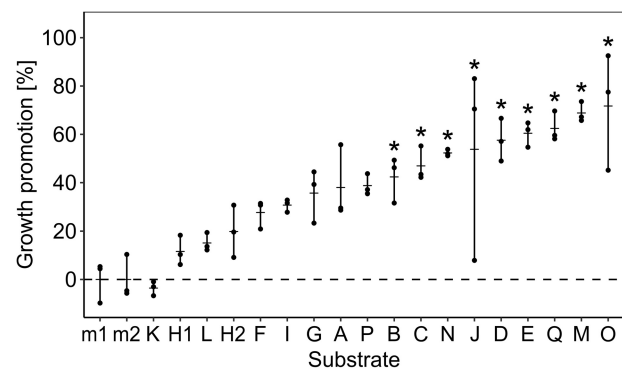
Figure 1. Growth promotion of cress plants due to compost applications. Percent growth promotion was measured as % increase in cress shoot weight compared with the matrix within each batch. Control (m1 and m2) and compost treatments (A–Q) were sorted in ascending order by their mean % growth promotion, and compost H was tested in both batches (H1 and H2) to assess the interbatch variability. Dashes and dots represent means and values of the replicates of each substrate, respectively. Asterisks indicate significant differences of compost treatments compared with both control matrices (Tukey HSD tests, P < 0.05 ). The dashed line shows 0% growth promotion, which corresponds to the mean cress biomass of the matrix (m1 and m2).
