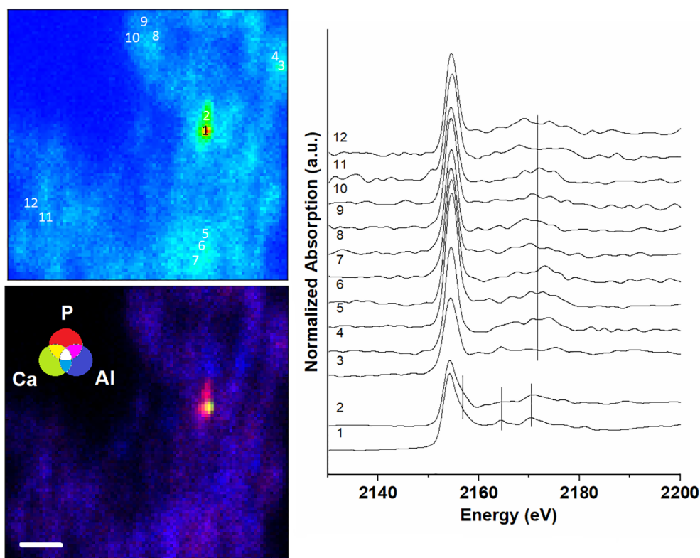
Fig. 2. XRF map of P, Ca and Al (left bottom; 0.7 μm step; color scale is arbitrary; white bar is 10 μm), P map with selected points of interest for micro-XANES (left top; red = high concentration, blue = low concentration), and micro-XANES spectra (right, vertical lines show features of same compound) of the soil sample 6A, analyzed at ID21 beamline, ESRF. The Ca-P grain shown on the map is approximately 5 \times 10 \mu\text{m}^2 . (For interpretation of the references to color in this figure legend, the reader is referred to the web version of this article.)
