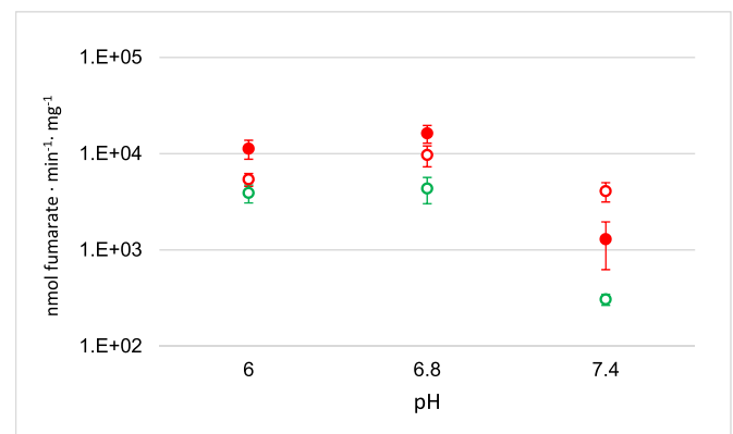
Fig. 4. Aspartase activity of recombinant aspartase. Aspartase activity at pH 6.0, pH 6.8, and pH 7.4 of recombinant aspartase AspA (green circle) from strain FAM14176, AspA1 (red circle), and AspA2 (full red circle) from Propionibacterium freudenreichii strain CIRM-BIA1. The vertical axis is logarithmically scaled.
